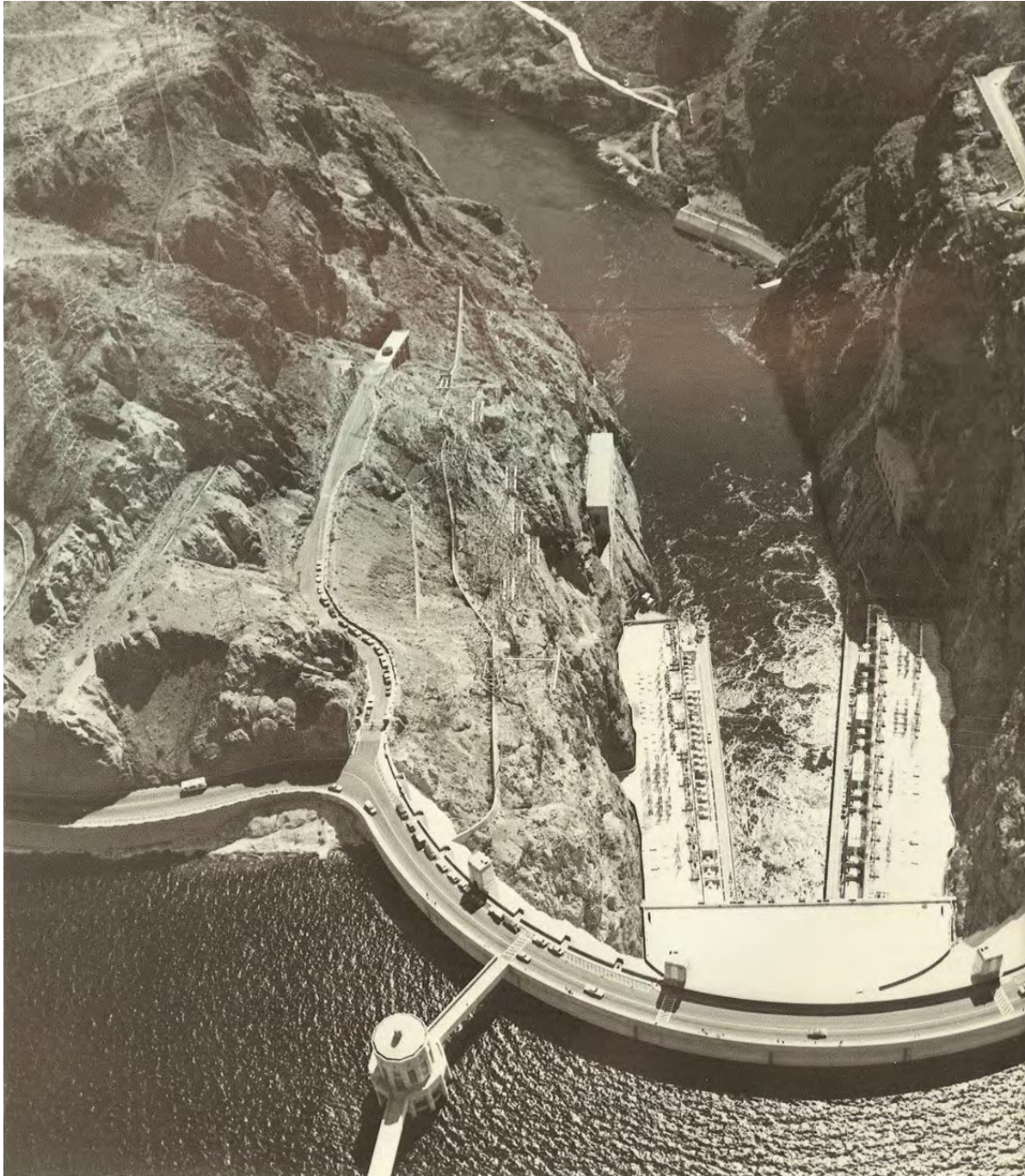
Aerial view of powerplant and Colorado River far below crest of Hoover Dam.
